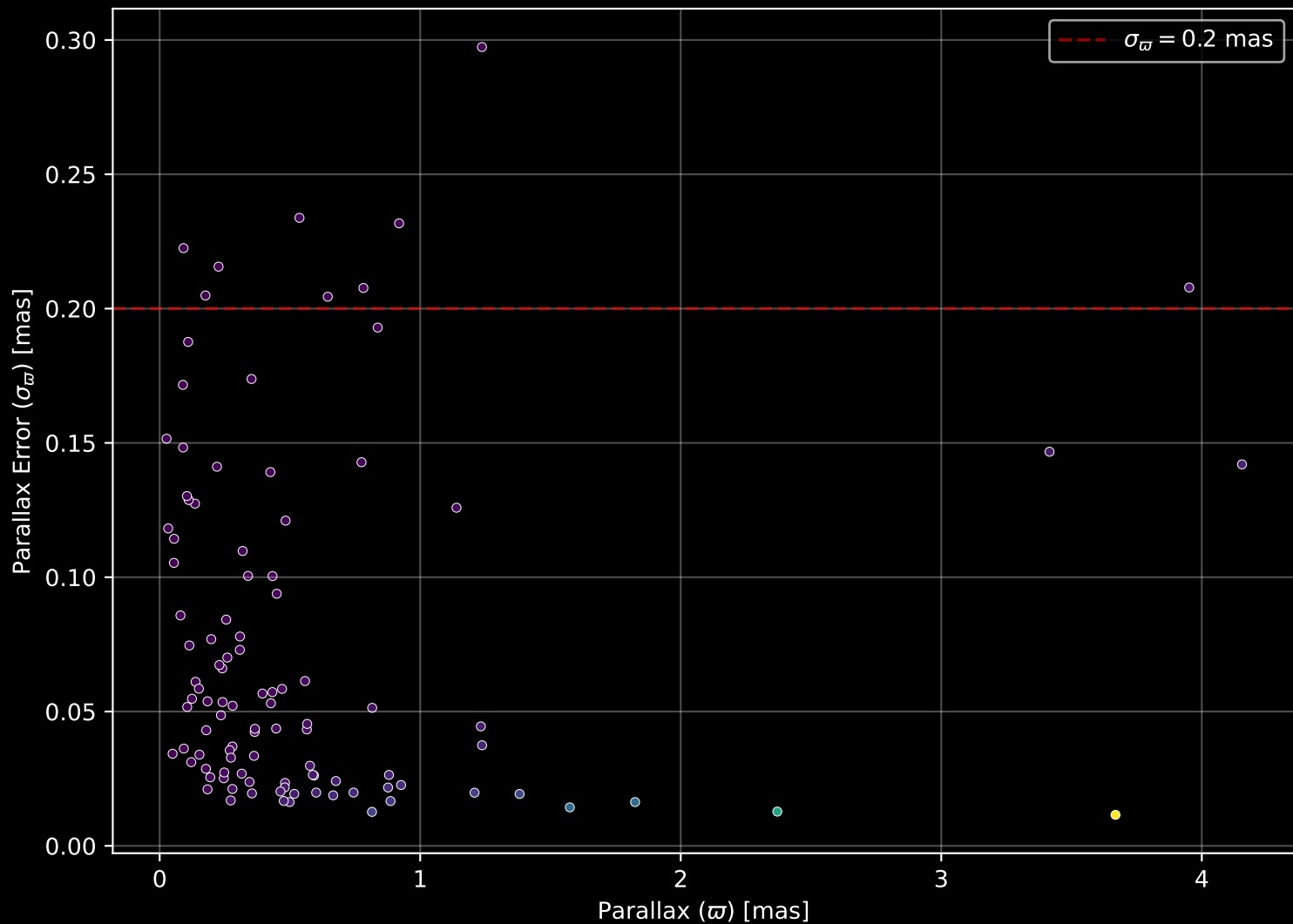
APOGEE DR17 Field: [305-00-C] Parallax Quality (n= 105)
