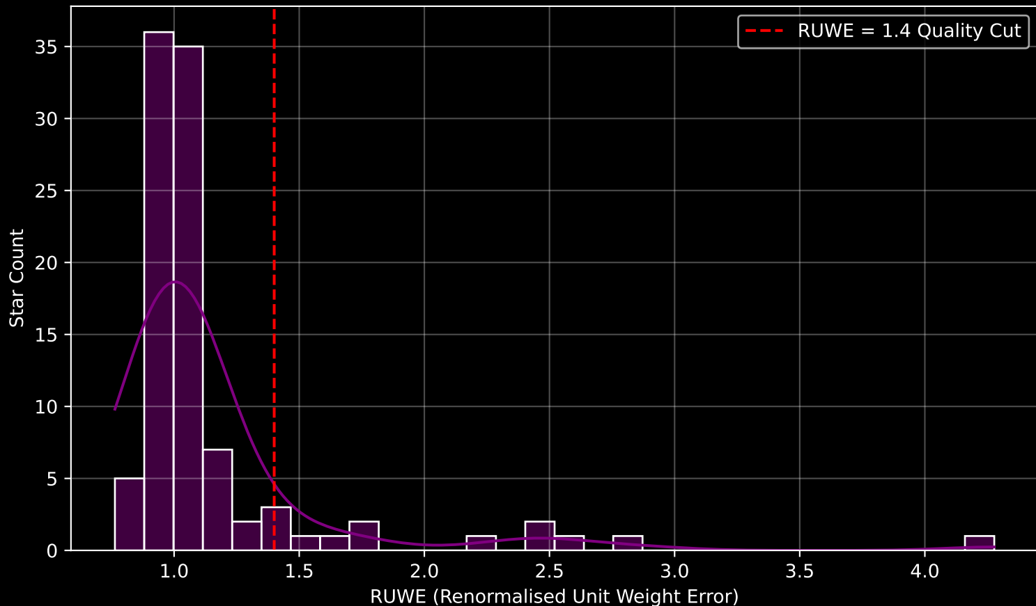
GAPOGEE DR17 Field [305-00-C] RUWE Distribution (n= 98)
