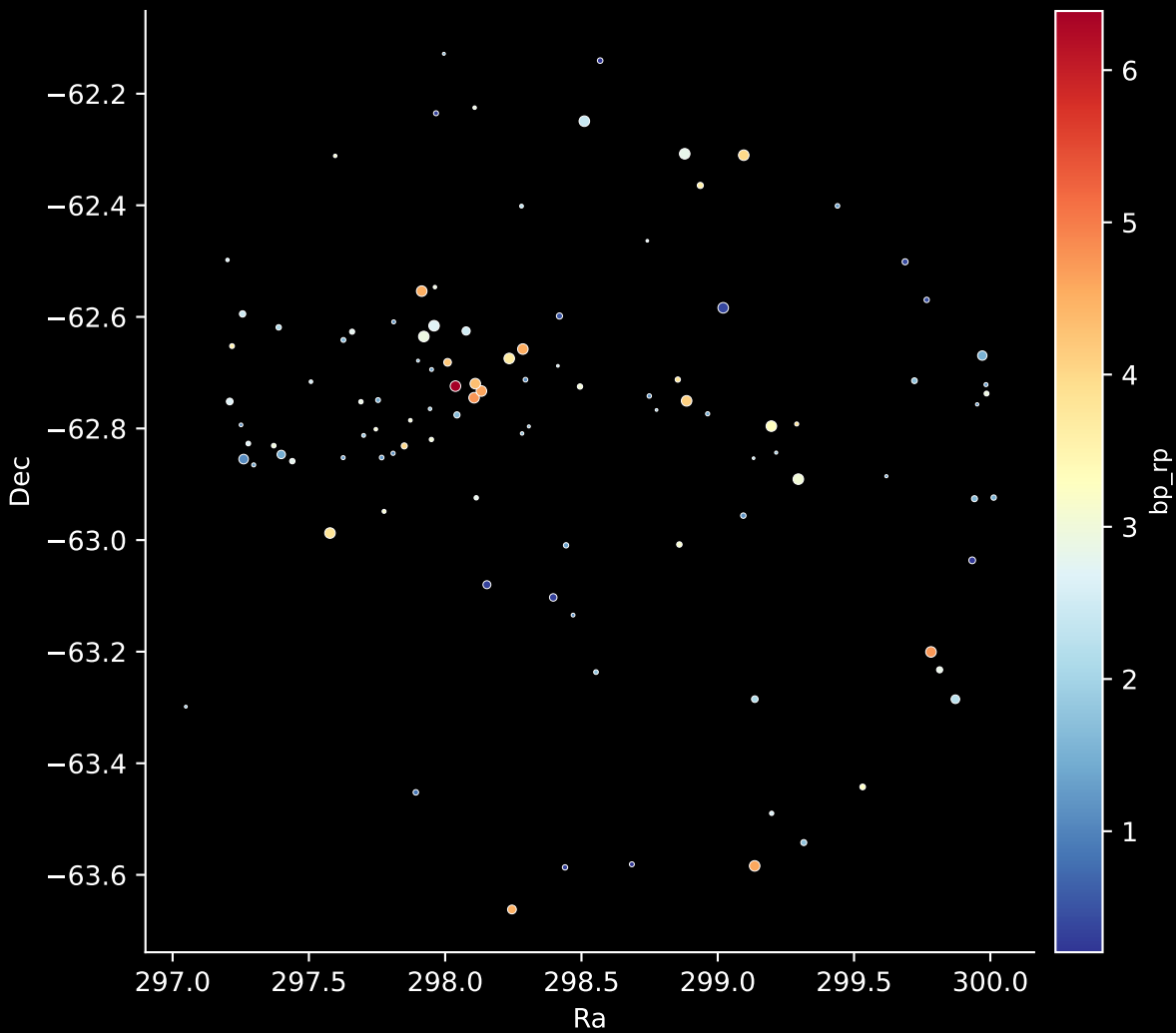
APOGEE DR17 Field: [305-00-C] Stars: 105
