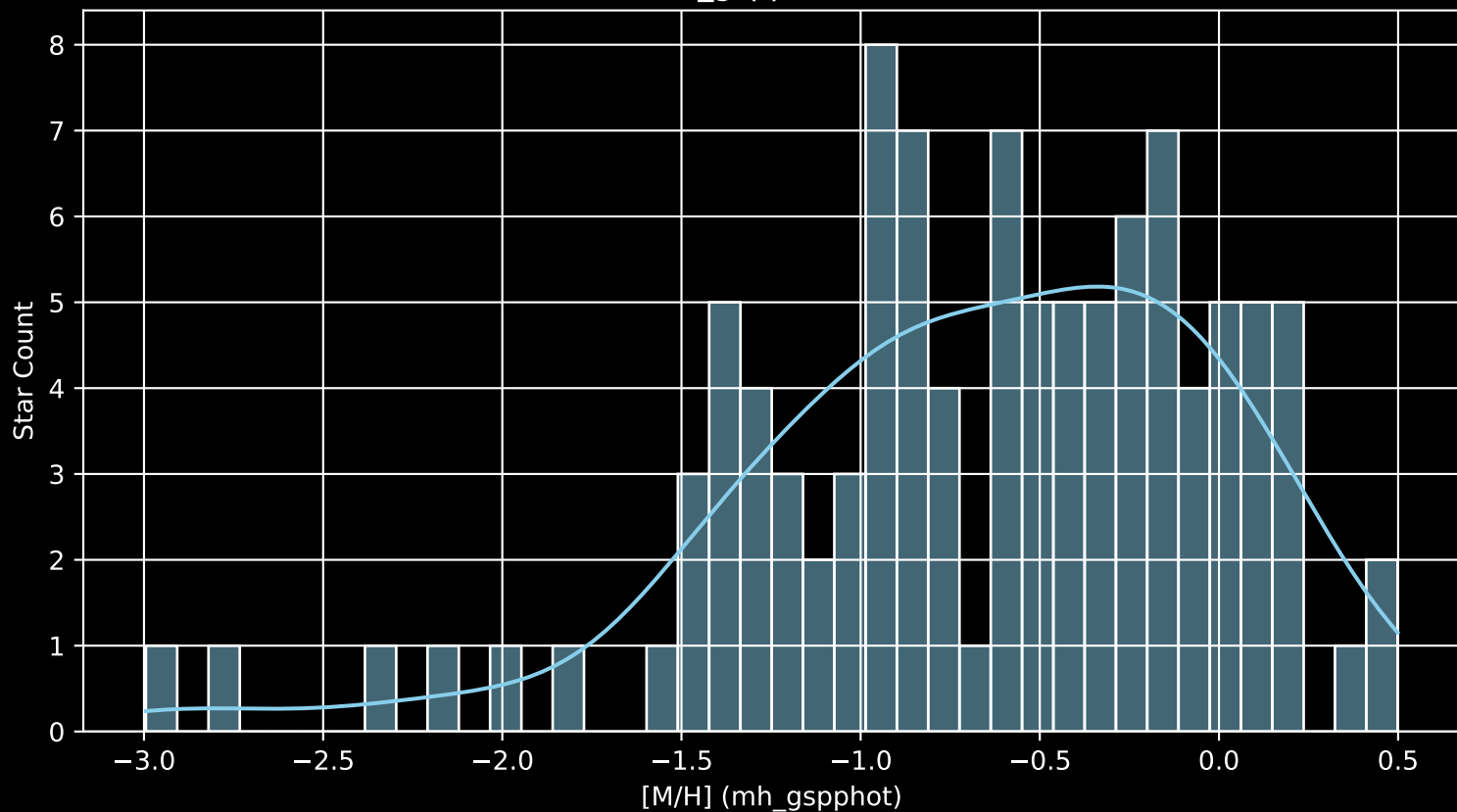
APOGEE DR17 Field: [305-00-C [M/H] (mh_gspphot) (n= 104)
