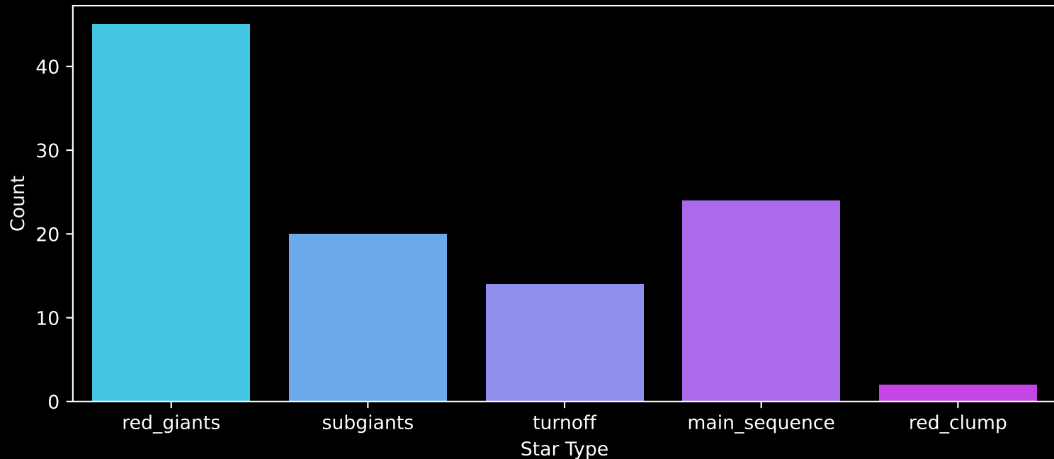
APOGEE DR17 Field: [305-00-C] Count plot of Star Type
