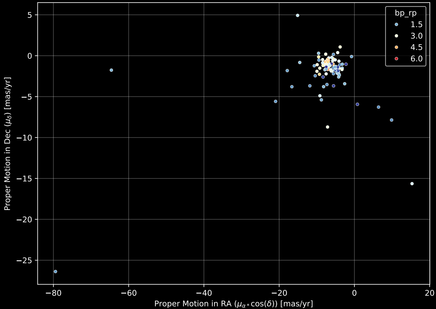
APOGEE DR17 Field: [305-00-C] Proper Motion Diagram (n= 105)
