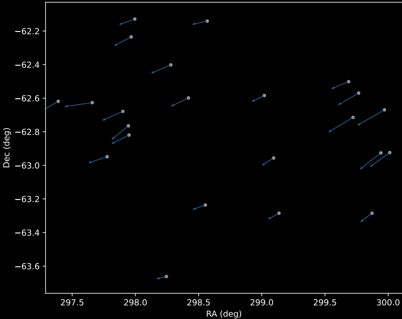
APOGEE DR17 Cluster 0 Proper Motion Vectors (n=23)
